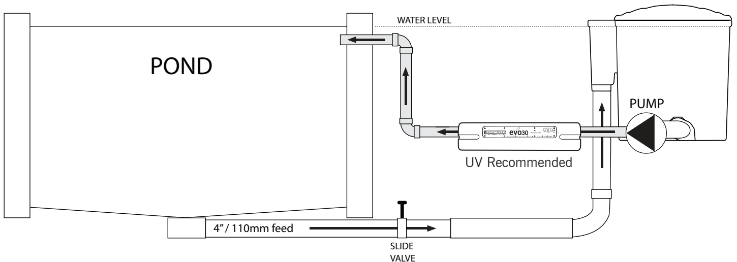
Figure 3. Gravity Fed System (Water gravity fed into Pod and returned to pond by pump)
